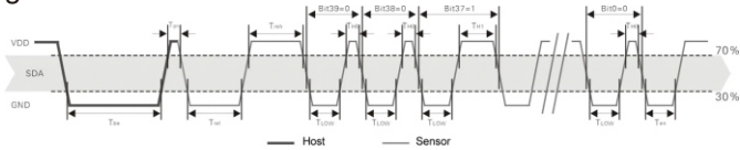
Figure 8 AM2302 Single bus communication timing
